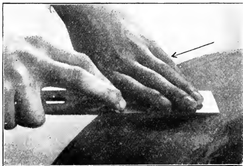
Fig. 115—Grinding Plane Iron
